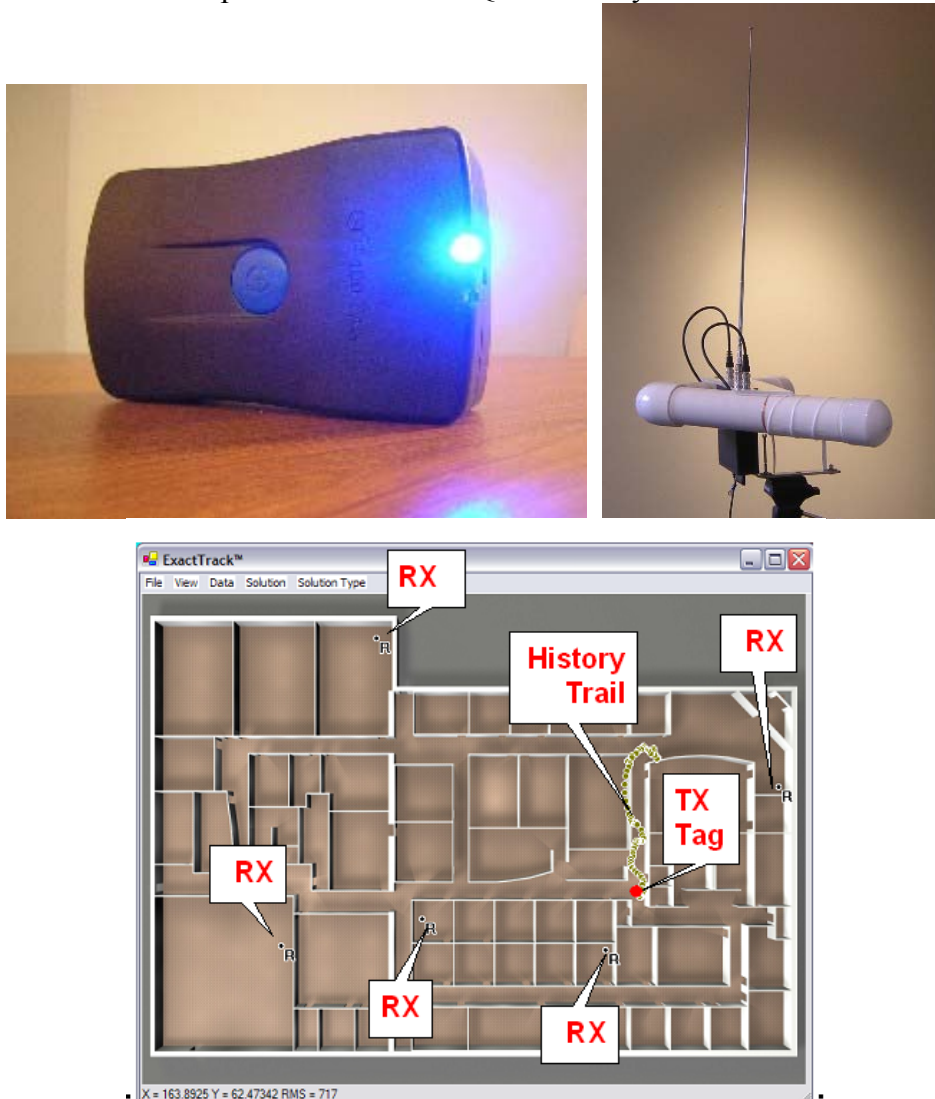
Figure 2a (top-left): A QT™-400 Tag Transmitter.
