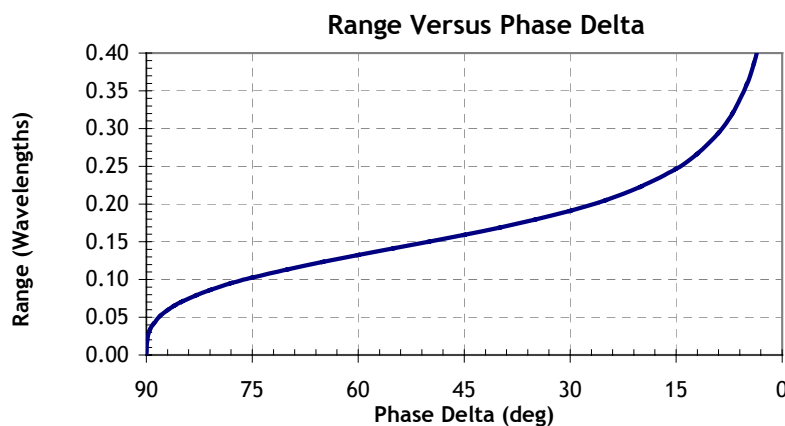
Figure 1: The phase delta between the electric and magnetic phase components provides useful range information within about one third of a wavelength of an electrically small antenna [© 2006, Q-Track].
