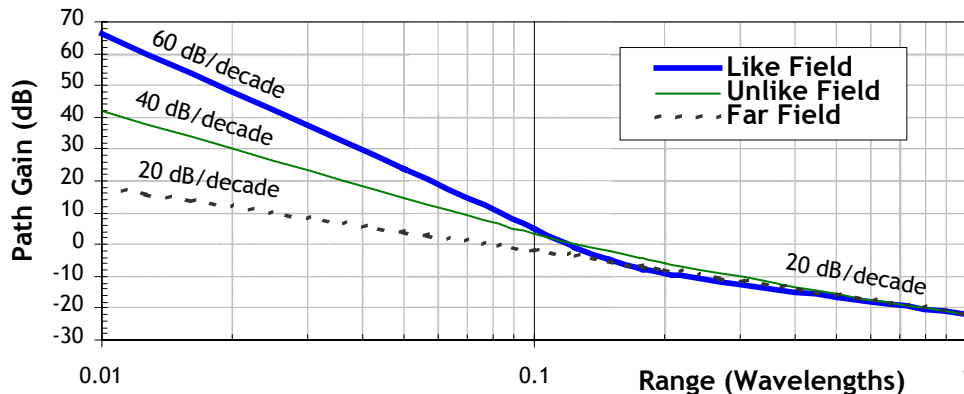
Figure 3: The near-field channel. In the near-field region (within \lambda/2\pi ), like links roll-off as the inverse sixth power (60dB/decade) and unlike links roll-off as the inverse fourth power (40dB/decade). In the far-field region, both like and unlike links converge to roll-off as the inverse square power (20dB/decade) described by the usual Friis Law [© 2006, Q-Track].
