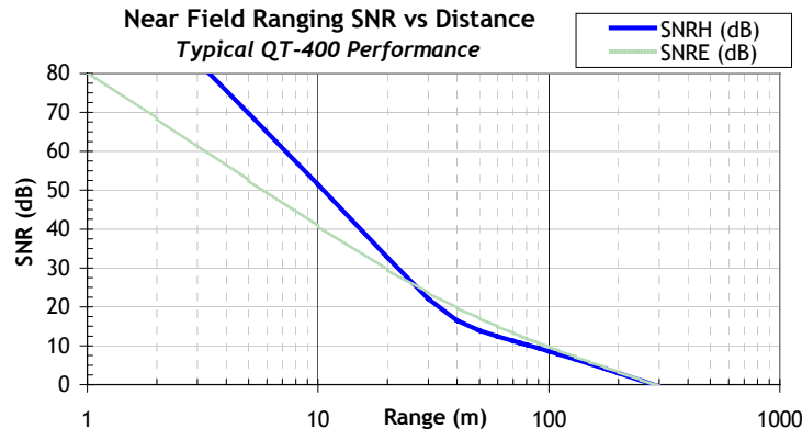
Figure 4: Typical SNR results for Q-Track's QT-400 Starter Kit System. [© 2006, Q-Track].
