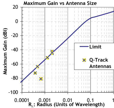
Figure 4(a) A matched pair of antennas with boundary spheres of radius R can be no closer than about d = 2R without their boundary spheres overlapping. (b) Limit on antenna gain vs. size showing a variety of Q-Track antennas [Q-Track; ©2004].
